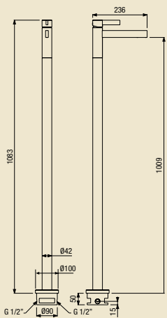
500030 _ _ Piantana a pavimento per lavabo. Floor mounted wash basin mixer.
