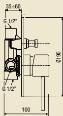
800033 __ Miscelatore monocomando incasso con deviatore. Wall-mounted single lever shower mixer, with diverter.
