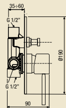
800033 __ Miscelatore monocomando lavabo a parete. Wall-mounted single lever shower mixer, without diverter.
